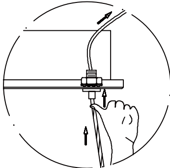
Shorten cable: Please hold down the bottom of the wire lock and slowly push or pull the cable upwards.
