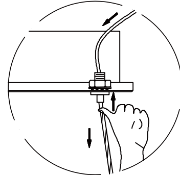
Stretching cable: Please hold down the bottom of the wire lock and slowly push or pull the cable down.
