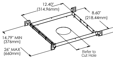
NEW CONSTRUCTION PLATE TRIM/TRIMLESS 43786-015
