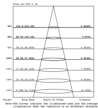
26W 1-LIGHT Round GIMBAL WIDE CLEAR
