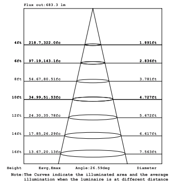
26W 1-LIGHT Round GIMBAL MEDIUM CLEAR
