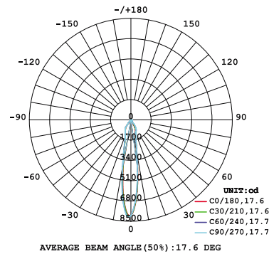
26W 1-LIGHT Round GIMBAL NARROW CLEAR
