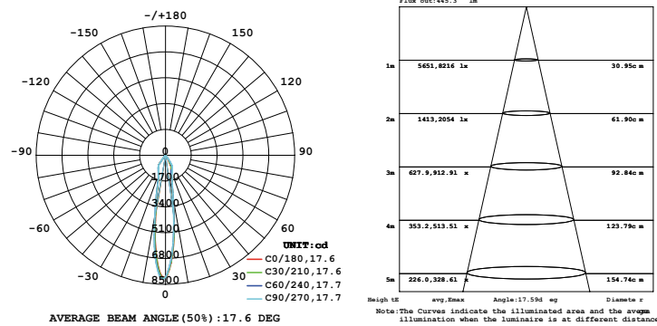
26W 1-LIGHT Round GIMBAL NARROW CLEAR
