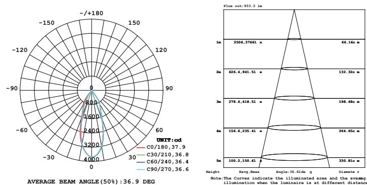
26W 1-LIGHT Round GIMBAL WIDE CLEAR
