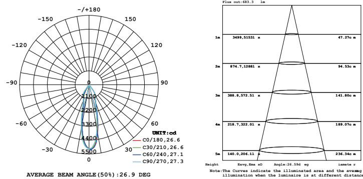
26W 1-LIGHT Round GIMBAL MEDIUM CLEAR
