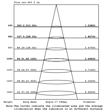
26W 1-LIGHT Round GIMBAL NARROW CLEAR
