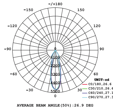
26W 1-LIGHT Round GIMBAL MEDIUM CLEAR
