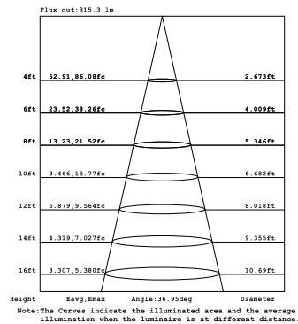
26W 1-LIGHT Round WALL WASH MEDIUM CLEAR
