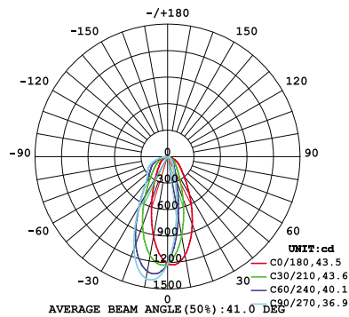
26W 1-LIGHT Round WALL WASH MEDIUM CLEAR
