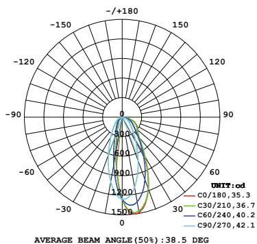
26W 1-LIGHT Round WALL WASH NARROW CLEAR
