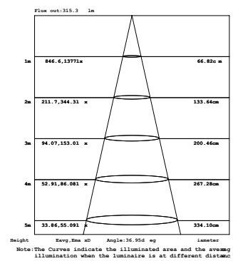
26W 1-LIGHT Round WALL WASH MEDIUM CLEAR
