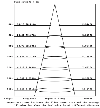
26W 1-LIGHT Round WALL WASH NARROW CLEAR
