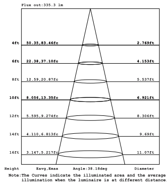
26W 1-LIGHT Round WALL WASH WIDE CLEAR
