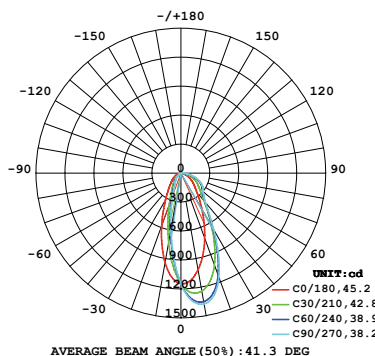
26W 1-LIGHT Round WALL WASH WIDE CLEAR
