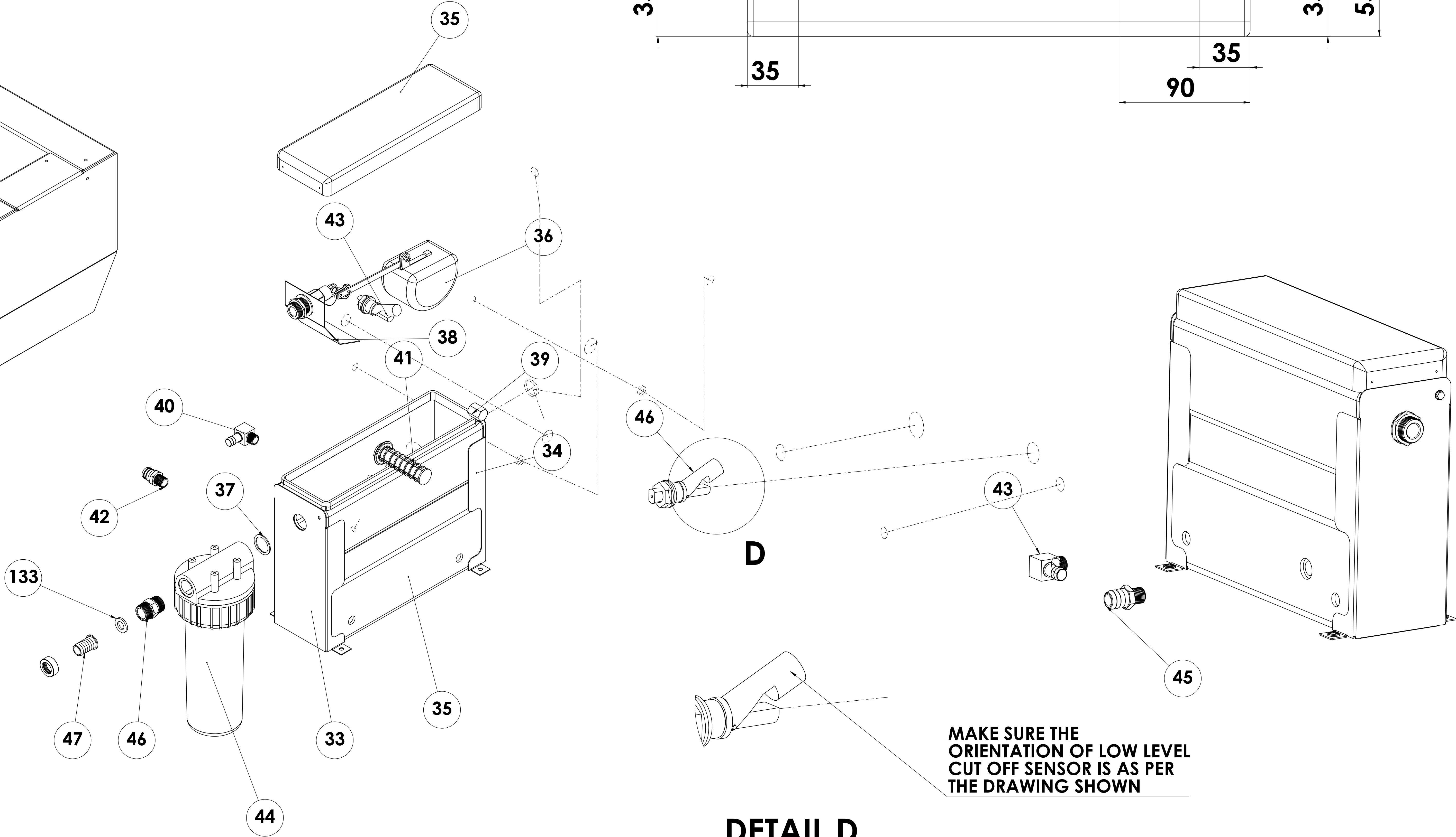
DETAIL D
