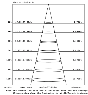
26W 1-LIGHT Square WALL WASH MEDIUM CLEAR
