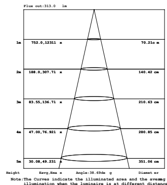
26W 1-LIGHT Square WALL WASH WIDE CLEAR
