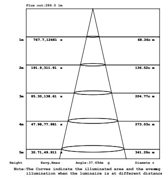
26W 1-LIGHT Square WALL WASH MEDIUM CLEAR
