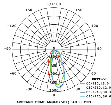
26W 1-LIGHT Square WALL WASH NARROW CLEAR
