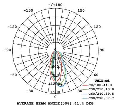
26W 1-LIGHT Square WALL WASH MEDIUM CLEAR
