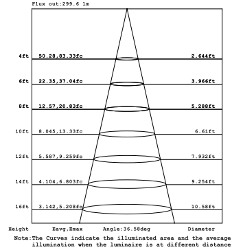
26W 1-LIGHT Square WALL WASH NARROW CLEAR
