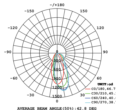
26W 1-LIGHT Square WALL WASH WIDE CLEAR
