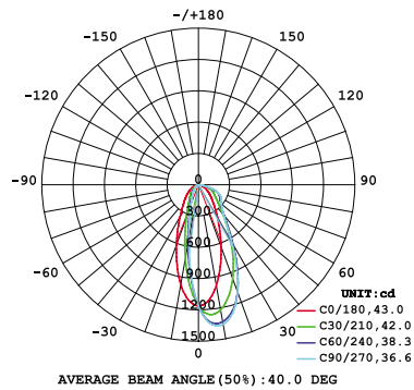
26W 1-LIGHT Square WALL WASH NARROW CLEAR
