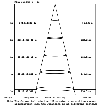
26W 1-LIGHT Square WALL WASH NARROW CLEAR
