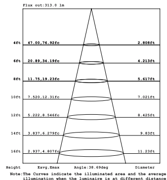
26W 1-LIGHT Square WALL WASH WIDE CLEAR
