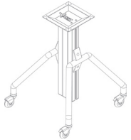
Arriba Omega Casters Base
