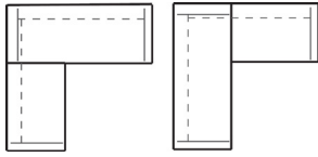
Elegante XT Worksurface - Left Return Two Piece L Shape Rectangle
