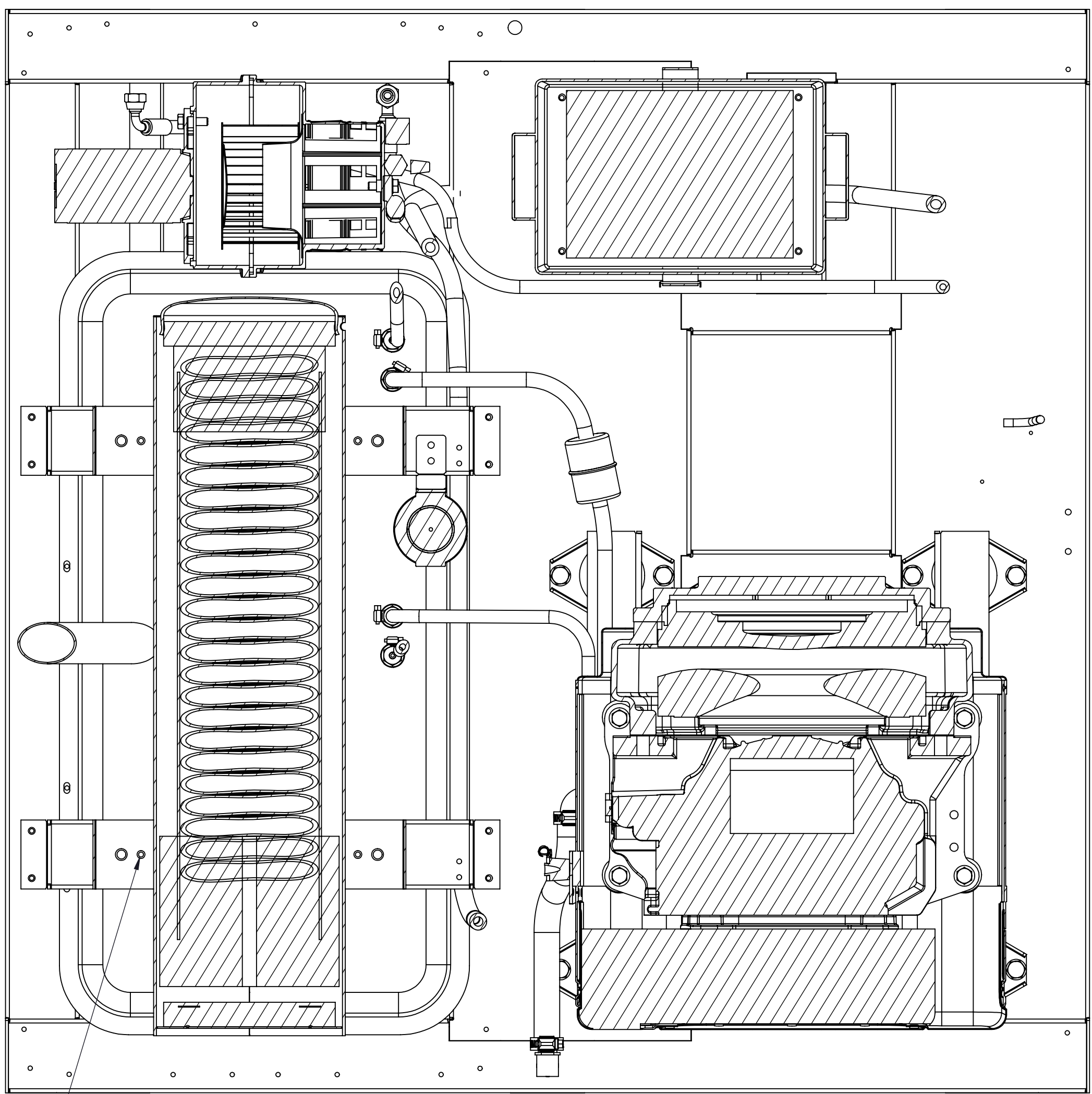
SECTION C-C
