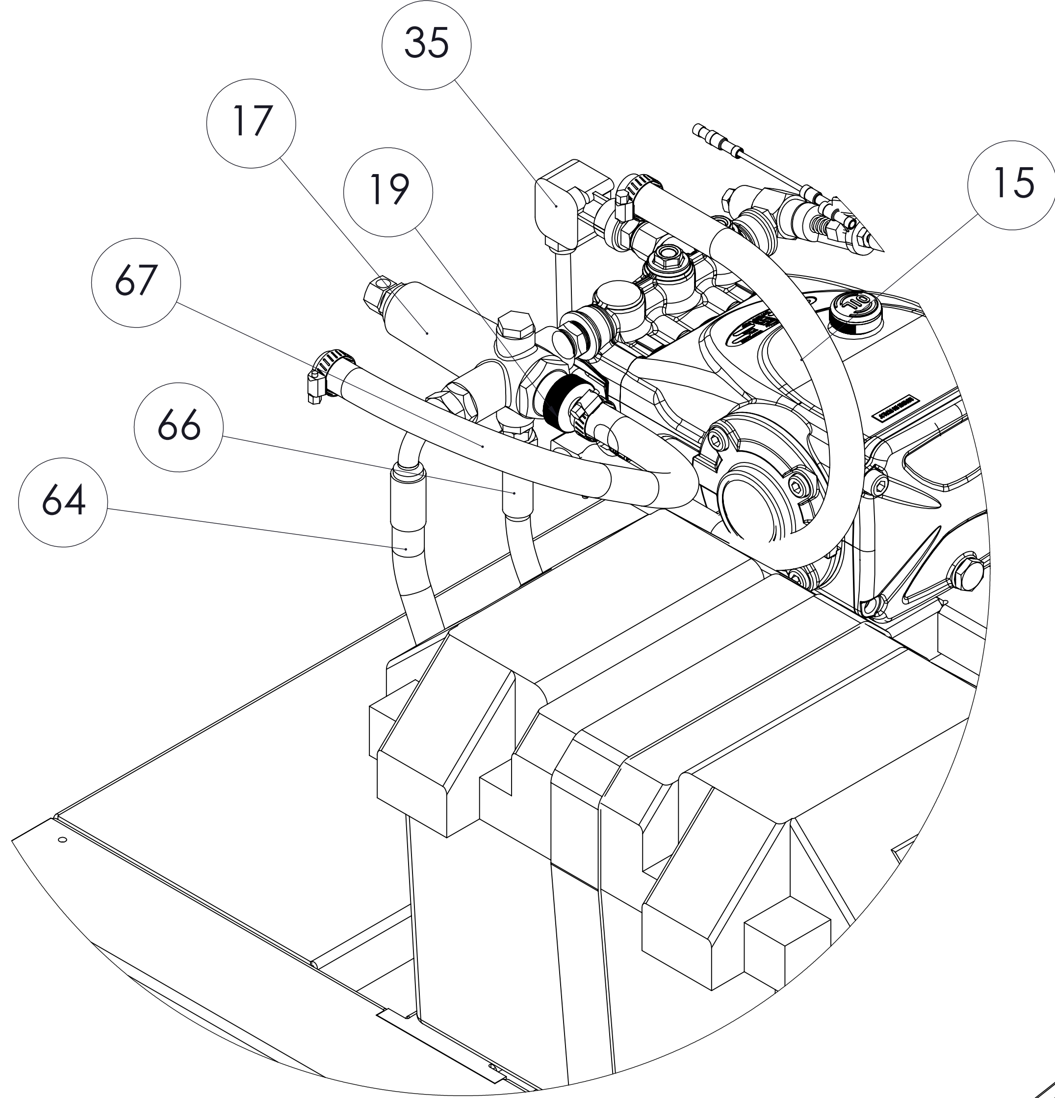
DETAIL B SCALE 1 : 2
