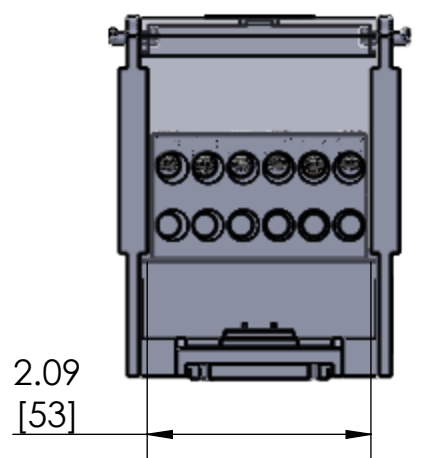
TAP SIDE
