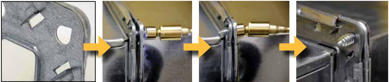
The teardrop shaped cut out of the corner with the proprietary bolt pull the connection together and lock it in place without the use of a nut, using a convenient cordless impact driver. Pictured above is the TDF® EZ Corner & 1" bolt.
