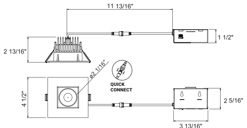
PRODUCT DIMENSIONS
