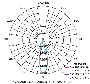
26W 1-LIGHT Square GIMBAL MEDIUM CLEAR
