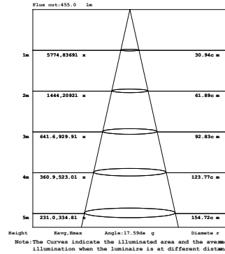
26W 1-LIGHT Square GIMBAL NARROW CLEAR
