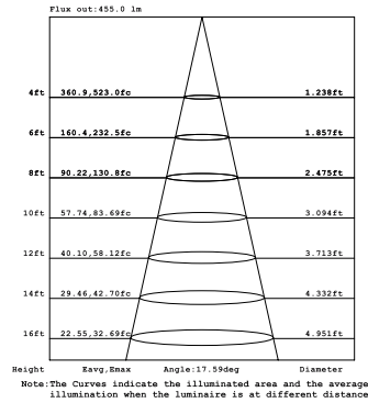
26W 1-LIGHT Square GIMBAL NARROW CLEAR
