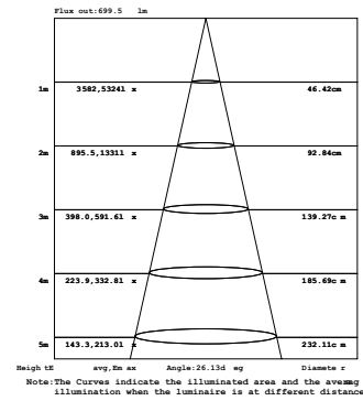
26W 1-LIGHT Square GIMBAL MEDIUM CLEAR
