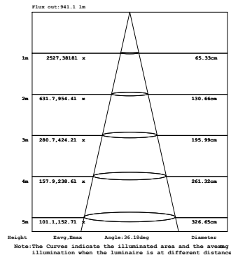
26W 1-LIGHT Square GIMBAL WIDE CLEAR
