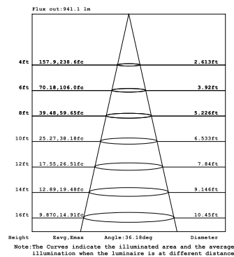
26W 1-LIGHT Square GIMBAL WIDE CLEAR
