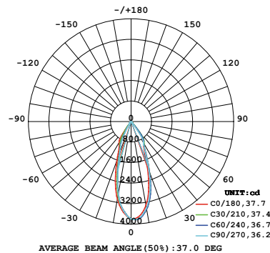
26W 1-LIGHT Square GIMBAL WIDE CLEAR
