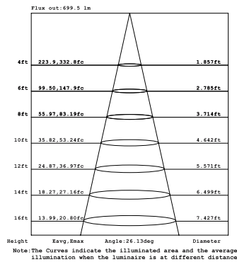
26W 1-LIGHT Square GIMBAL MEDIUM CLEAR
