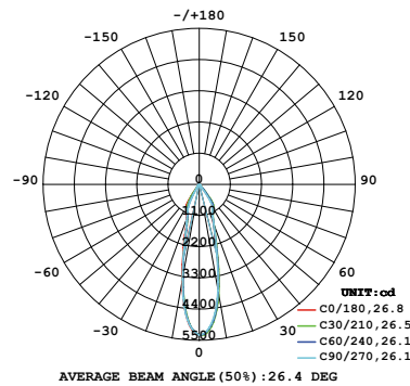
26W 1-LIGHT Square GIMBAL MEDIUM CLEAR
