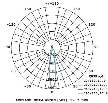
26W 1-LIGHT Square GIMBAL NARROW CLEAR
