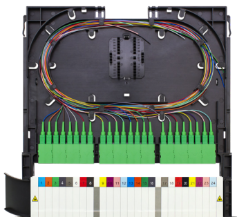
BladeHD™/Cassettes loaded with fiber pigtails
