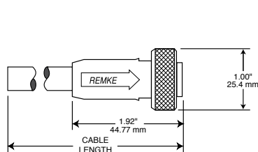
STRAIGHT PLUG
