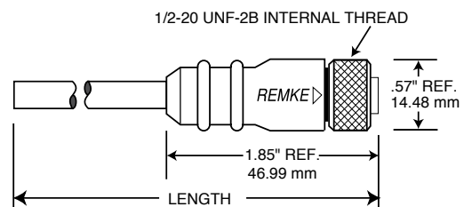
FEMALE STRAIGHT
