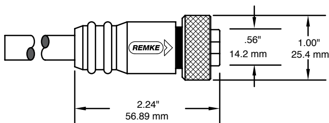
TYPICAL STRAIGHT
