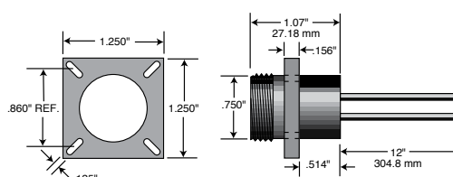
RECEPTACLE WITH FLANGE
