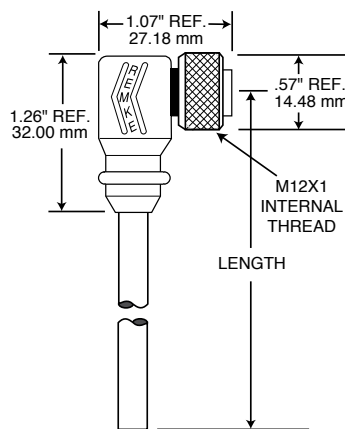
FEMALE 90 DEGREE
