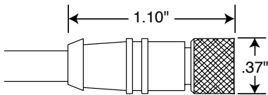
FEMALE STRAIGHT
