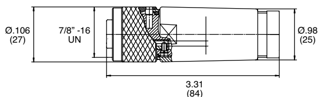
FEMALE STRAIGHT
