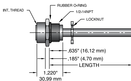
FEMALE RECEPTACLE
