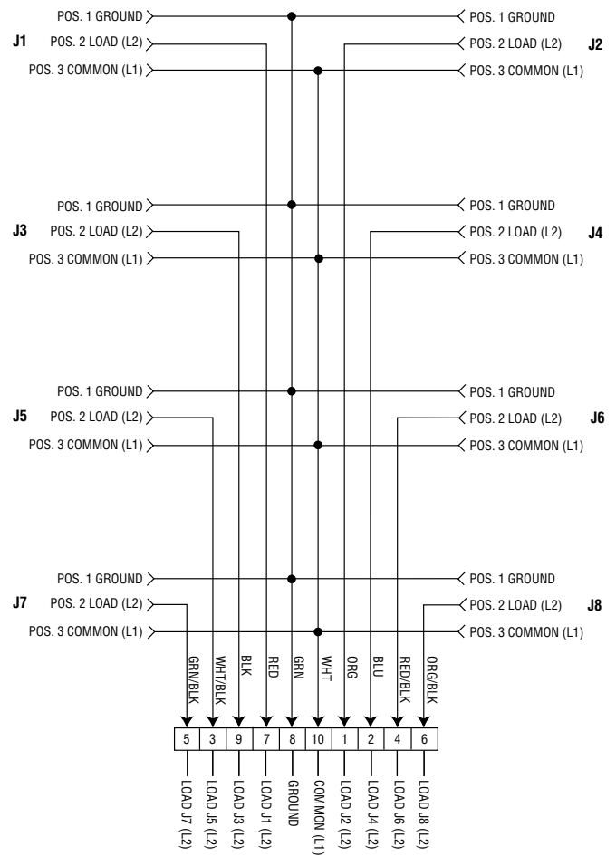
8 OUTLET WIRING SCHEMATIC
