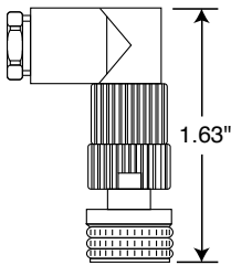
FEMALE 90°
