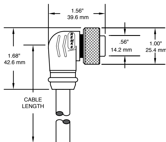
TYPICAL 90 DEGREE
