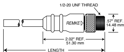
MALE STRAIGHT
