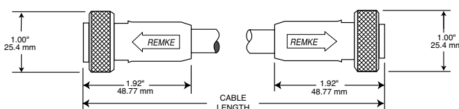
MALE/FEMALE CORDSET
