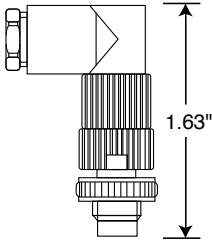
MALE 90°
