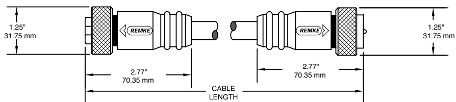
MALE/FEMALE CORDSET
