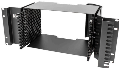
BladeHD™ Chassis
