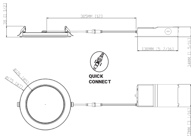
PRODUCT DIMENSIONS
