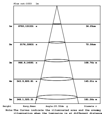
40W 1-LIGHT SquareDownlight NARROW CLEAR
