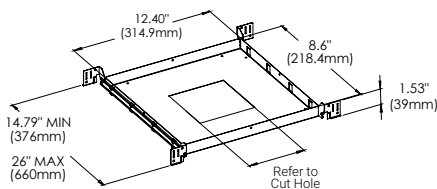
NEW CONSTRUCTION PLATE TRIM/TRIMLESS 24051-019
