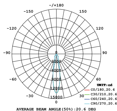
40W 1-LIGHT SquareDownlight NARROW CLEAR
