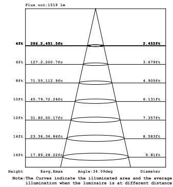
40W 1-LIGHT Square Downlight WIDE CLEAR
