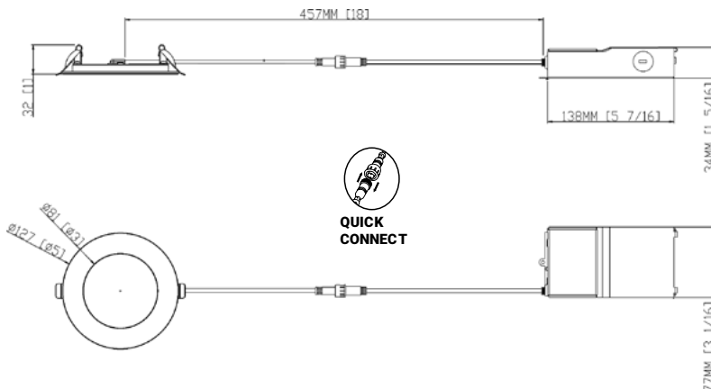
PRODUCT DIMENSIONS
