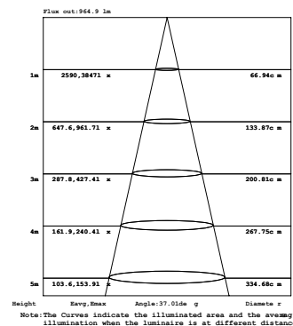
26W 1-LIGHT Square DOWNLIGHT WIDE CLEAR
