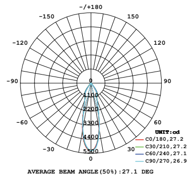
26W 1-LIGHT Square DOWNLIGHT MEDIUM CLEAR
