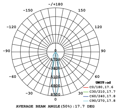
26W 1-LIGHT Square DOWNLIGHT NARROW CLEAR
