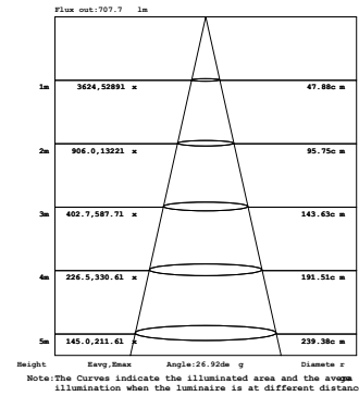
26W 1-LIGHT Square DOWNLIGHT MEDIUM CLEAR
