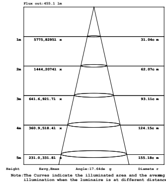
26W 1-LIGHT Square DOWNLIGHT NARROW CLEAR
