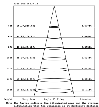
26W 1-LIGHT Square DOWNLIGHT WIDE CLEAR
