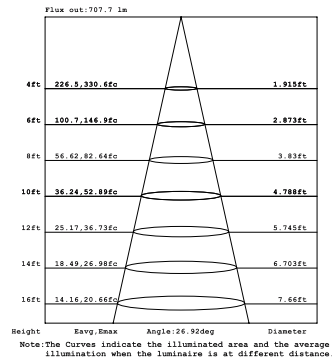
26W 1-LIGHT Square DOWNLIGHT MEDIUM CLEAR
