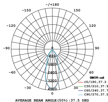
26W 1-LIGHT Square DOWNLIGHT WIDE CLEAR
