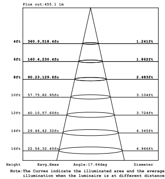
26W 1-LIGHT Square DOWNLIGHT NARROW CLEAR
