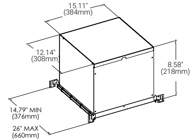
TRIM AT/IC Box: 46749-017
