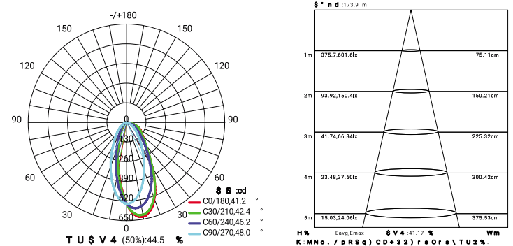
15W 1-LIGHT WALL WASH WIDE CLEAR
