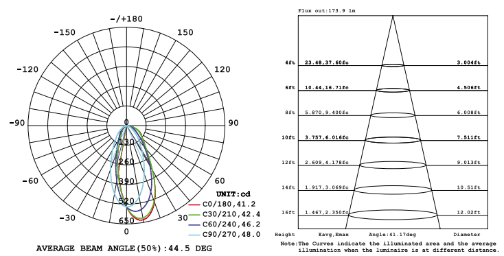
15W 1-LIGHT WALL WASH WIDE CLEAR
