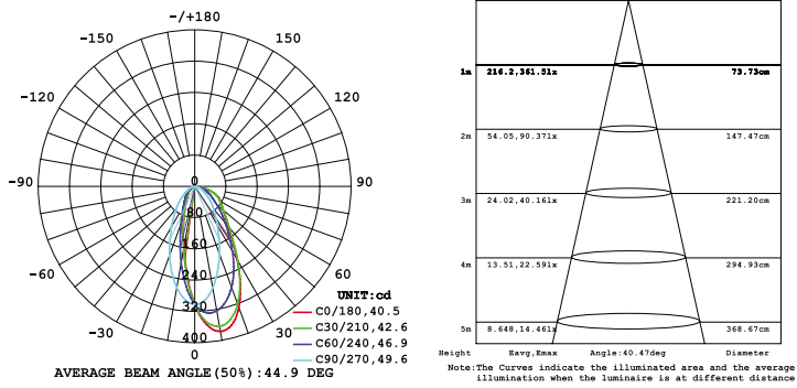
10W 1-LIGHT WALL WASH WIDE CLEAR
