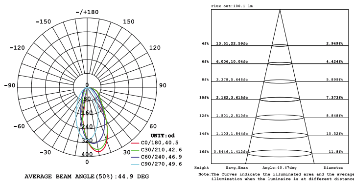
10W 1-LIGHT WALL WASH WIDE CLEAR
