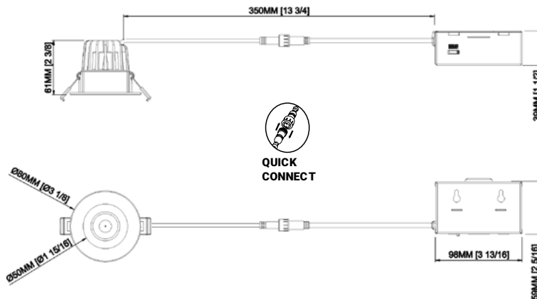
PRODUCT DIMENSIONS
