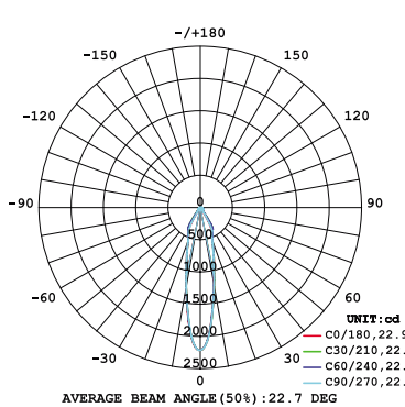
10W 1-LIGHT Square DOWNLIGHT MEDIUM CLEAR
