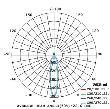
15W 1-LIGHT Square DOWNLIGHT MEDIUM CLEAR
