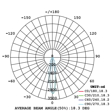
10W 1-LIGHT Square DOWNLIGHT NARROW CLEAR
