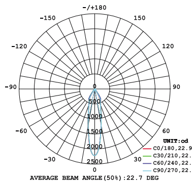
10W 1-LIGHT Square DOWNLIGHT MEDIUM CLEAR
