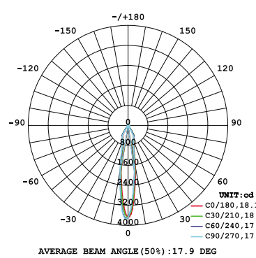
15W 1-LIGHT Square DOWNLIGHT NARROW CLEAR
