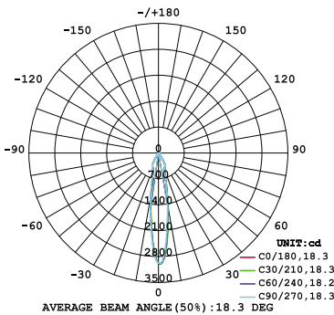
10W 1-LIGHT Square DOWNLIGHT NARROW CLEAR
