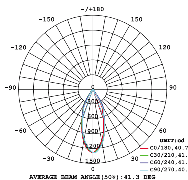
10W 1-LIGHT Square DOWNLIGHT WIDE CLEAR
