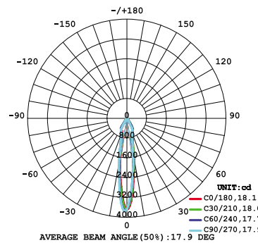
15W 1-LIGHT Square DOWNLIGHT NARROW CLEAR
