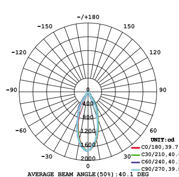
15W 1-LIGHT Square DOWNLIGHT WIDE CLEAR
