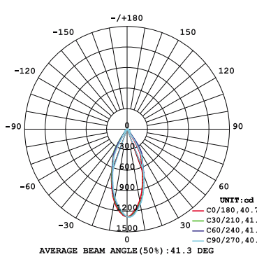
10W 1-LIGHT Square DOWNLIGHT WIDE CLEAR
